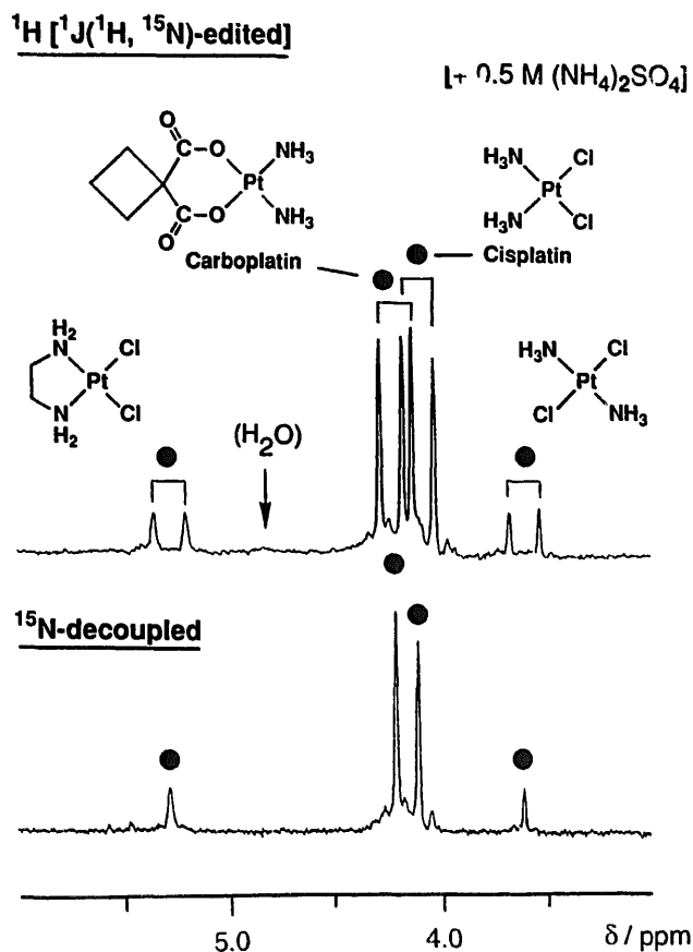
Fig. 8. ^1\text{H}\{-^{15}\text{N}\} NMR spectra of cisplatin (1), transplatin, carboplatin (2) and [\text{Pt}(\text{en})\text{Cl}_2] in 95% \text{H}_2\text{O} –5% \text{D}_2\text{O} . This method detects only protons bound to ^{15}\text{N} and in the top spectrum these appear as doublets due to ^{15}\text{N} coupling. The bottom spectrum is ^{15}\text{N} decoupled and each different type of NH appears as a singlet (along with broadened ^{195}\text{Pt} satellites). In this example ammonium sulphate was added as a relaxation agent to improve water suppression, but a similar suppression could also be achieved using pulsed field gradients.
